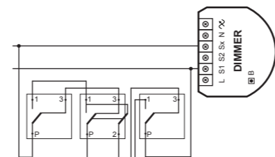
Fig.4 Example of 3-way switch connection
