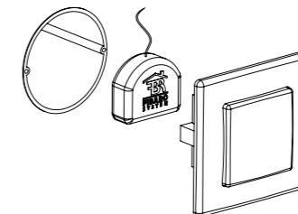
Fig.6 Installation of Fibaro Dimmer in a wall switch box.
