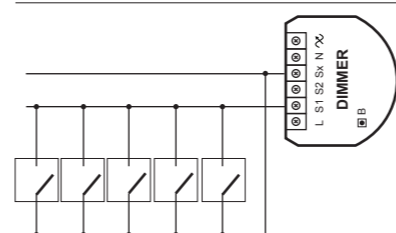
Fig.5 Example of momentary wall switches connection
