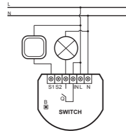
Double switch - mains electricity power connection
